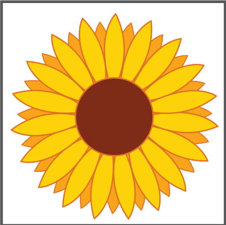
11. WRINKLE TOOL
