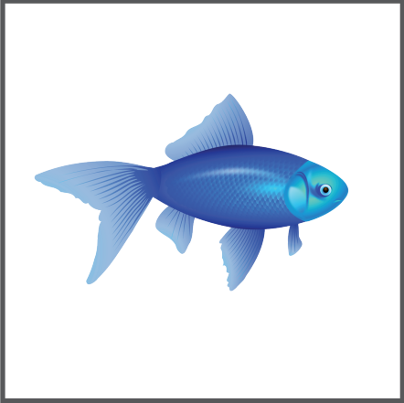
5. WARP TOOL
