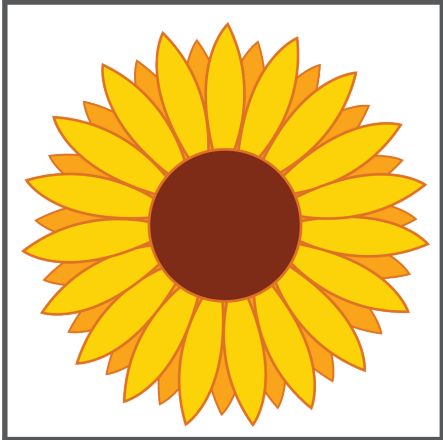
10. CRYSTALLIZE TOOL
